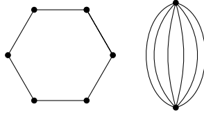
FIGURE 3. The cycle and banana graphs C_n and B_n for n = 6 .
