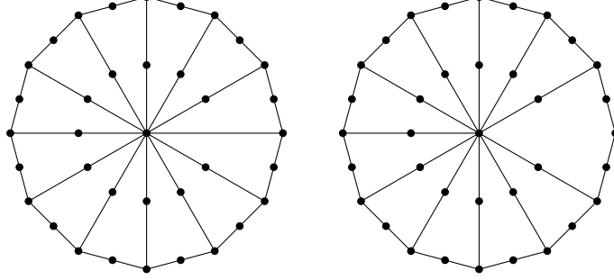
FIGURE 6. The graphs \widehat{W}_n/f and \widehat{W}_n \setminus \{e, f\} for n = 12 .
