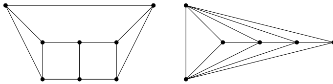
FIGURE 2. The graph G and its dual G^\perp .
