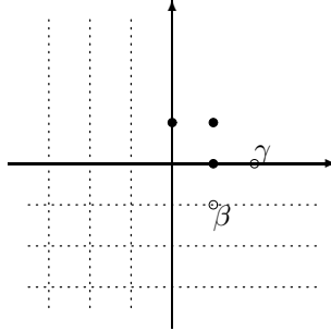
FIGURE 1. A and \text{sRes}(A) (dotted) in Example 4.1
