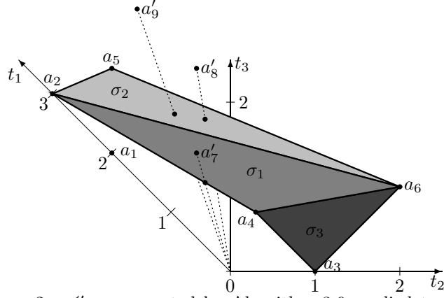
FIGURE 2. \mathcal{A}' as generated by Algorithm 3.9 applied to Example 3.15 and its central projection onto the (\mathcal{A}, \mathbf{1}) -umbrella
