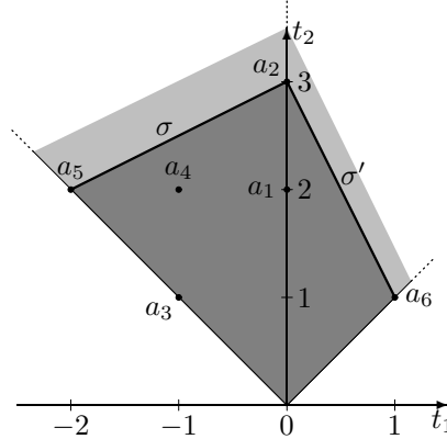
FIGURE 4. The (\mathcal{A}, \mathbf{1}) -polyhedron for Example 4.2
