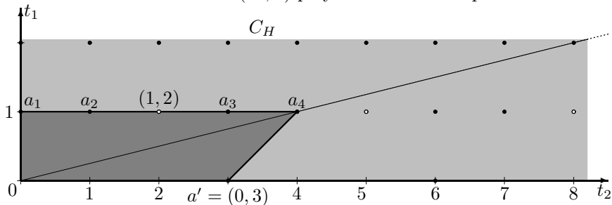
FIGURE 3. The (\mathcal{A}, 1) -polyhedron for Example 4.1
