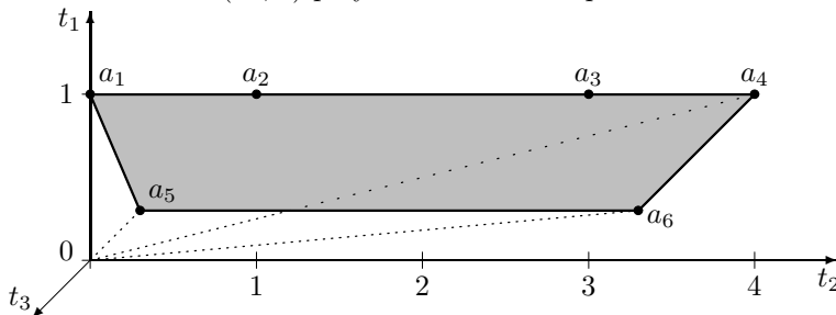
FIGURE 1. The (\mathcal{A}, 1) -polyhedron for Example 2.5
